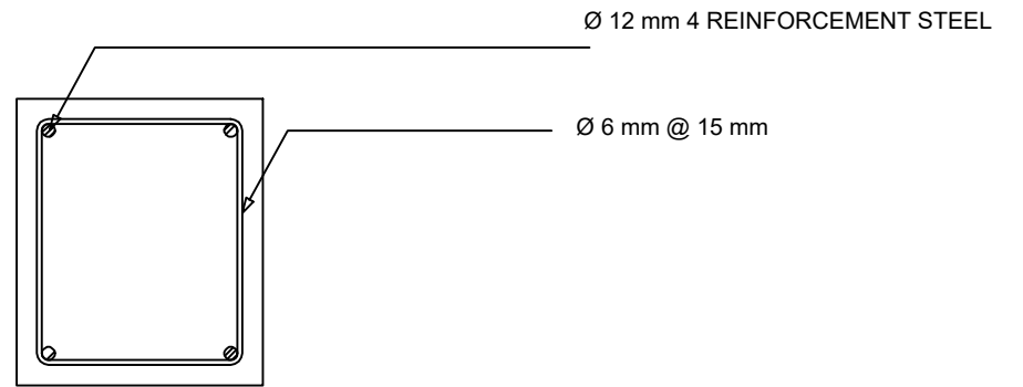
TIE BEAM DETAIL
