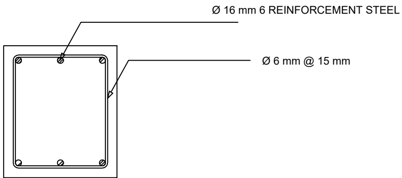
GRADE BEAM DETAIL
